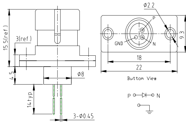
Package Dimensions
